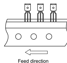
No. YF003-A-Z-SD-1.0
