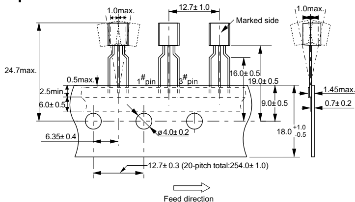
No. YS003-A-P-SD-1.0
