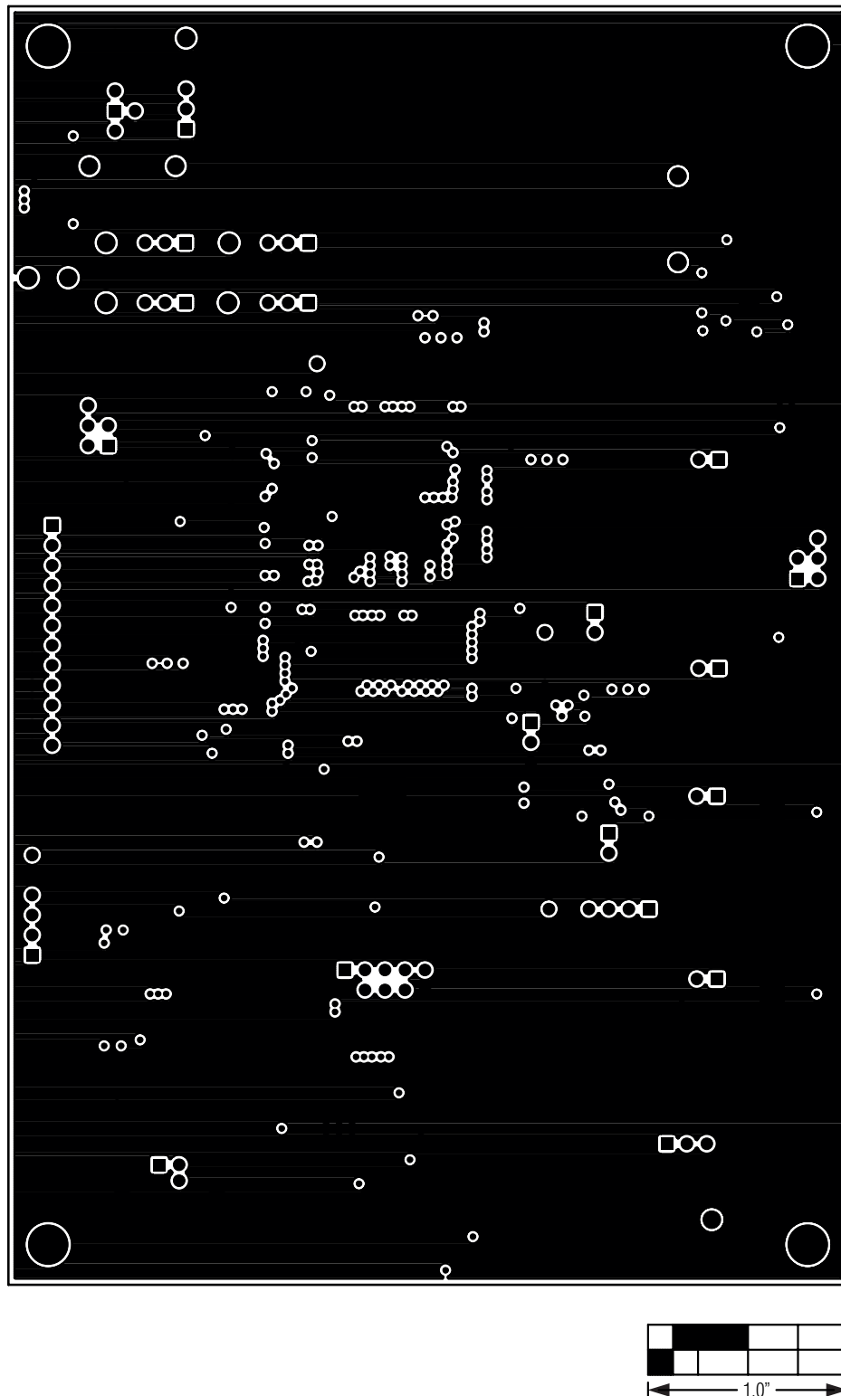
Figure 8. MAX44000 EV Kit PCB Layout—Layer 2
