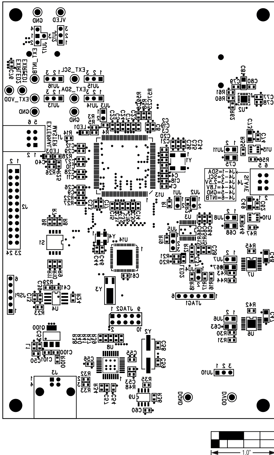
Figure 11. MAX44000 EV Kit Component Placement Guide—Bottom
