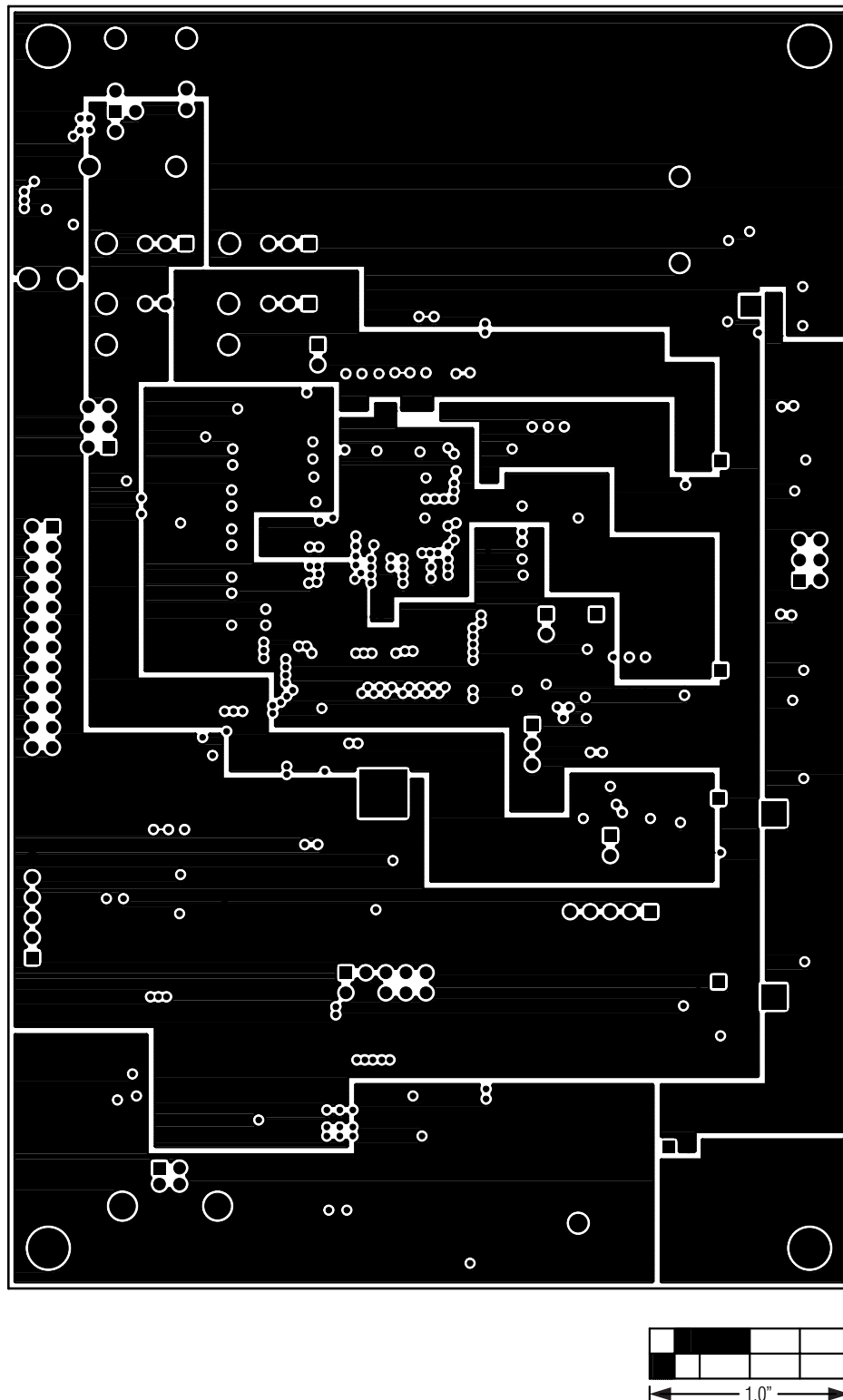
Figure 9. MAX44000 EV Kit PCB Layout—Layer 3
