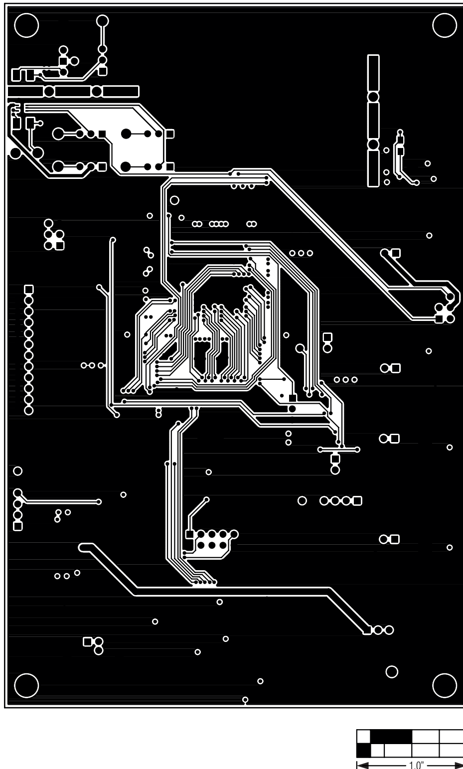
Figure 7. MAX44000 EV Kit PCB Layout—Component Side
