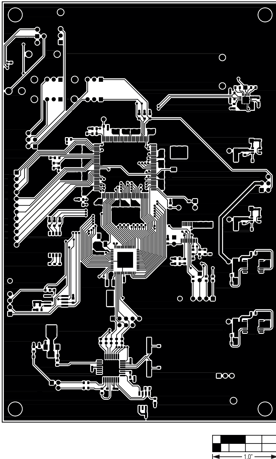
Figure 10. MAX44000 EV Kit PCB Layout—Bottom Side
