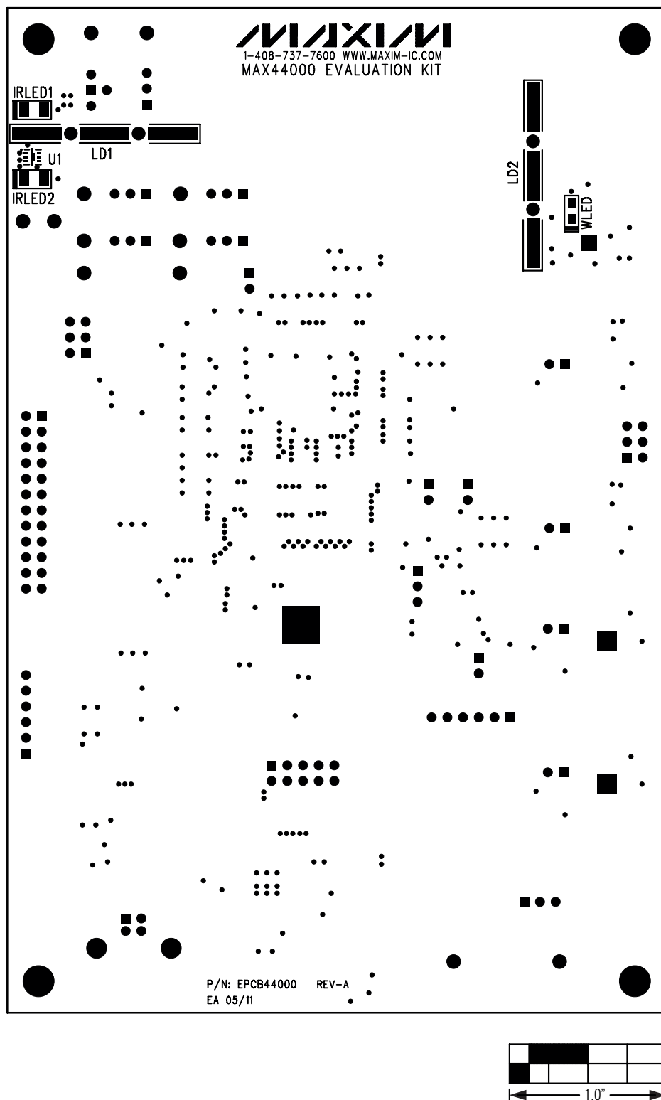
Figure 6. MAX44000 EV Kit Component Placement Guide—Component Side
