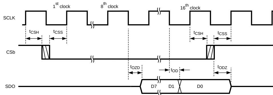
Figure 23. Read Timing
