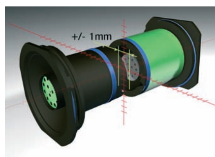
Axial alignment
