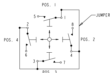
(C) SPST-NO 4 WAY WITH COMMON JUMPER SCHEMATIC
