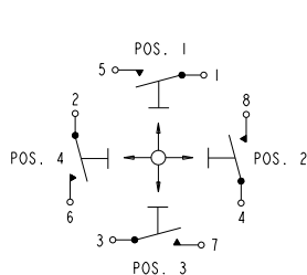
(C) SPST-NO 4 WAY SCHEMATIC
