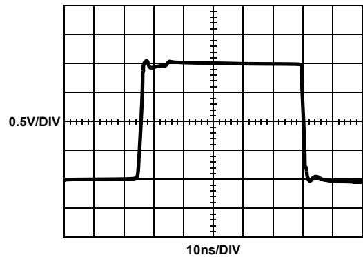
FIGURE 20. LARGE SIGNAL TRANSIENT RESPONSE
