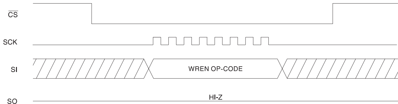
Figure 5. WRDI Timing
