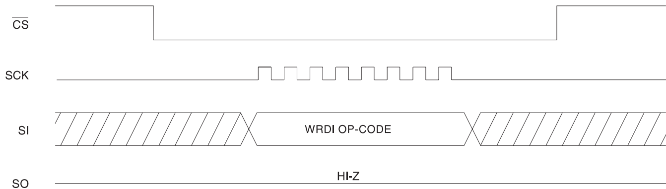
Figure 4. WREN Timing
