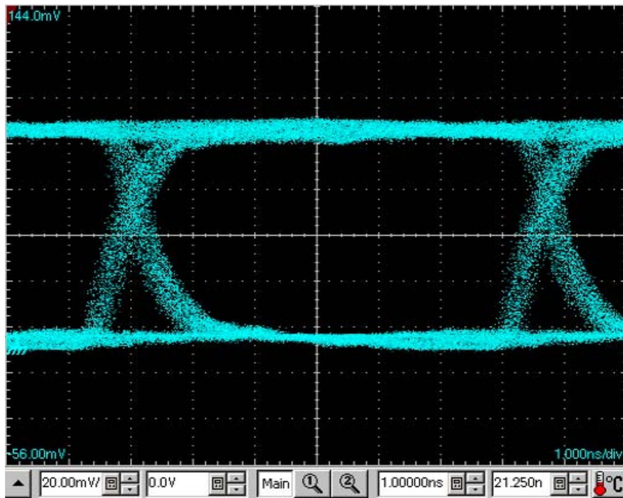
Figure 6. Eye Diagram
