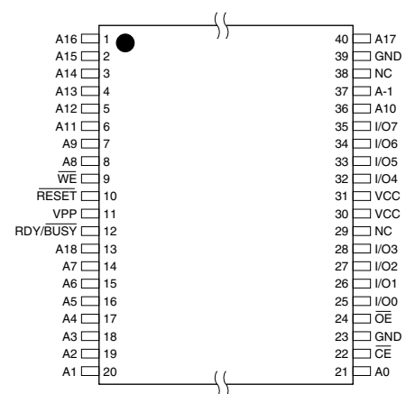
AT49BV008A(T) TSOP Top View
