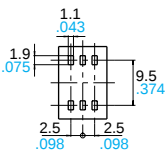
Recommended PC board pattern (TOP VIEW 2:1)
