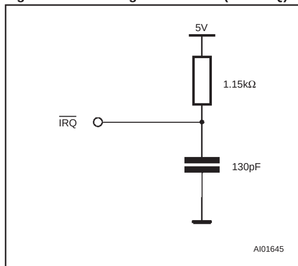
Figure 8. AC Testing Load Circuit (with \overline{\text{IRQ}} )
