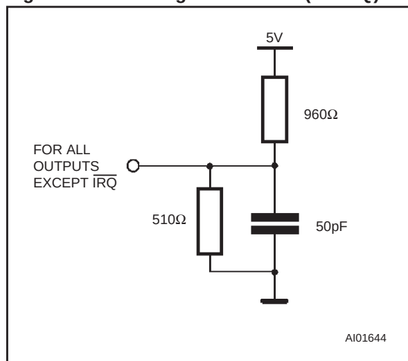
Figure 7. AC Testing Load Circuit (No \overline{\text{IRQ}} )
