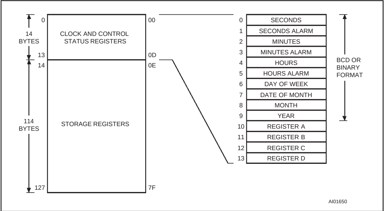
Figure 12. Address Map
