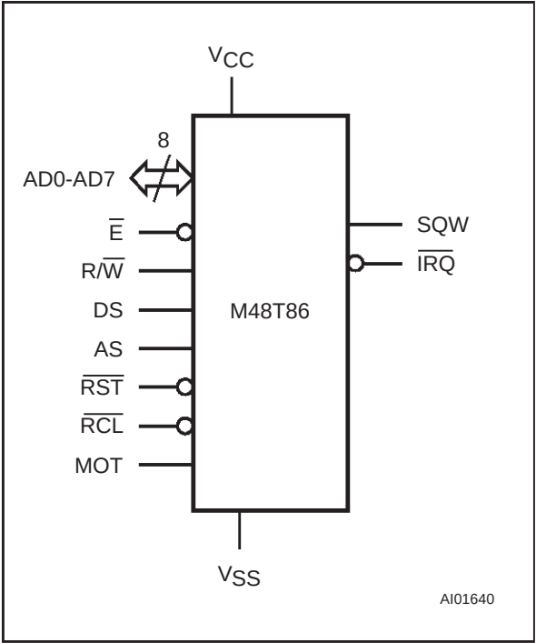
Figure 3. Logic Diagram
