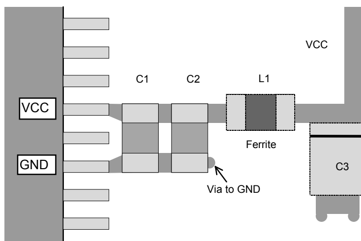
Figure 21. Decoupling and Bypass Capacitor Placement
