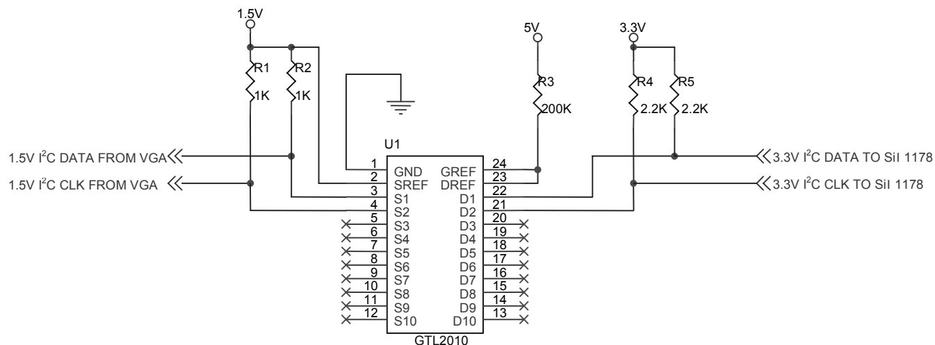
Figure 18. I²C Bus Voltage Level Shifting using Philips GTL 2010
