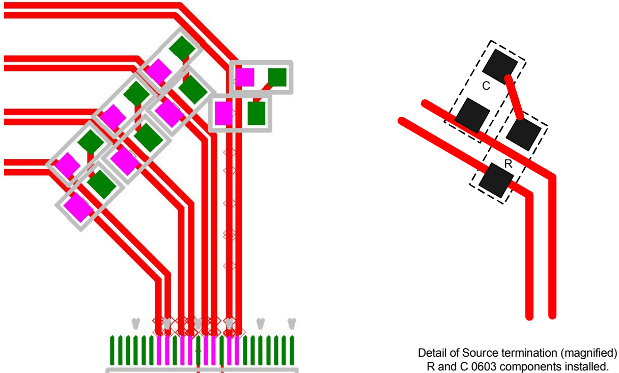
Figure 24. Source Termination Layout Illustration
