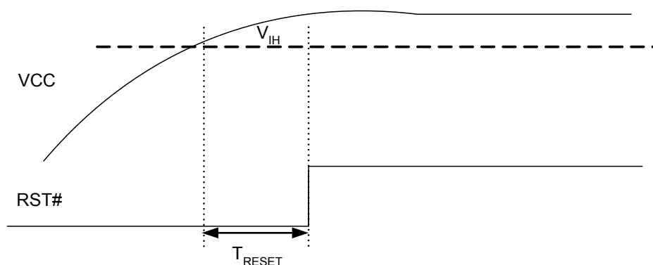
Figure 10. RST# Minimum Timing
