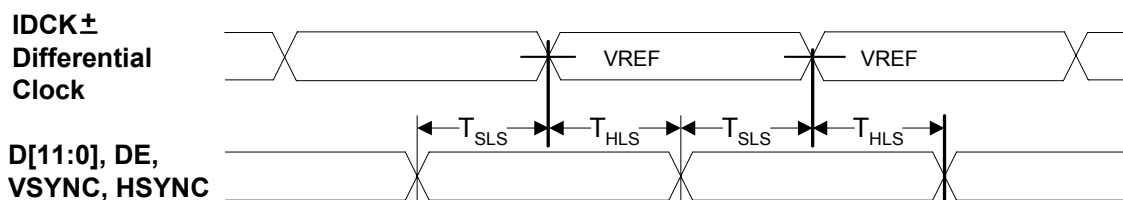
Figure 7. Low Swing Control and Data Setup/Hold Times to IDCK_{\pm} Differential Clock
