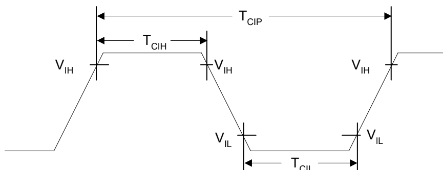
Figure 3. Clock Cycle/High/Low Times in High Swing Mode
