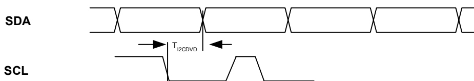
Figure 9. I²C Data Valid Delay (driving Read Cycle data)
