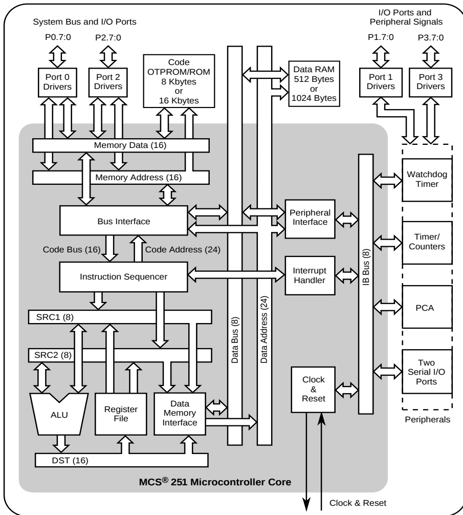
Figure 1. 8xC251TB/TQ Block Diagram
