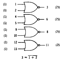
MC1010P, MC1011P, MC1012P MC1210P, MC1211P, MC1212F Quad 2-Input Gate
