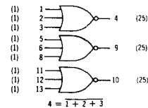
MC1007P, MC1008P, MC1009P MC1207F, MC1208F, MC1209F Triple 3-Input Gate
