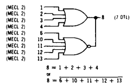
MC1018P, MC1218F Level Translator
