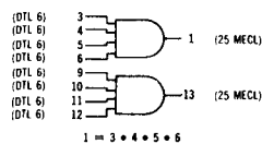
MC1017P, MC1217F Level Translator
