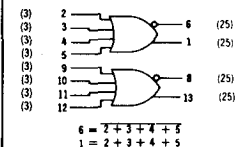
MC1023P Dual 4-Input Clock Driver
