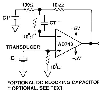
Figure 34. A Piezoelectric Transducer
