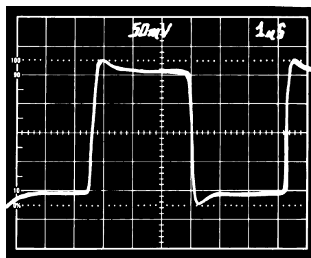
Figure 22b. Unity-Gain Follower Small Signal Pulse Response
