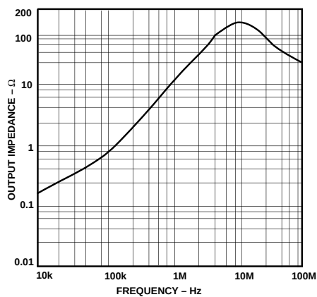
Figure 6. Output Impedance vs. Frequency (Closed Loop Gain = -1)
