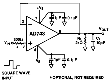
Figure 21. Unity-Gain Follower
