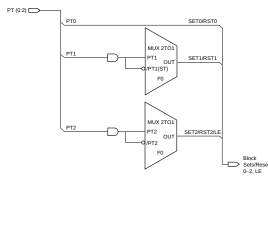
Figure 5. Set/Reset Generator
