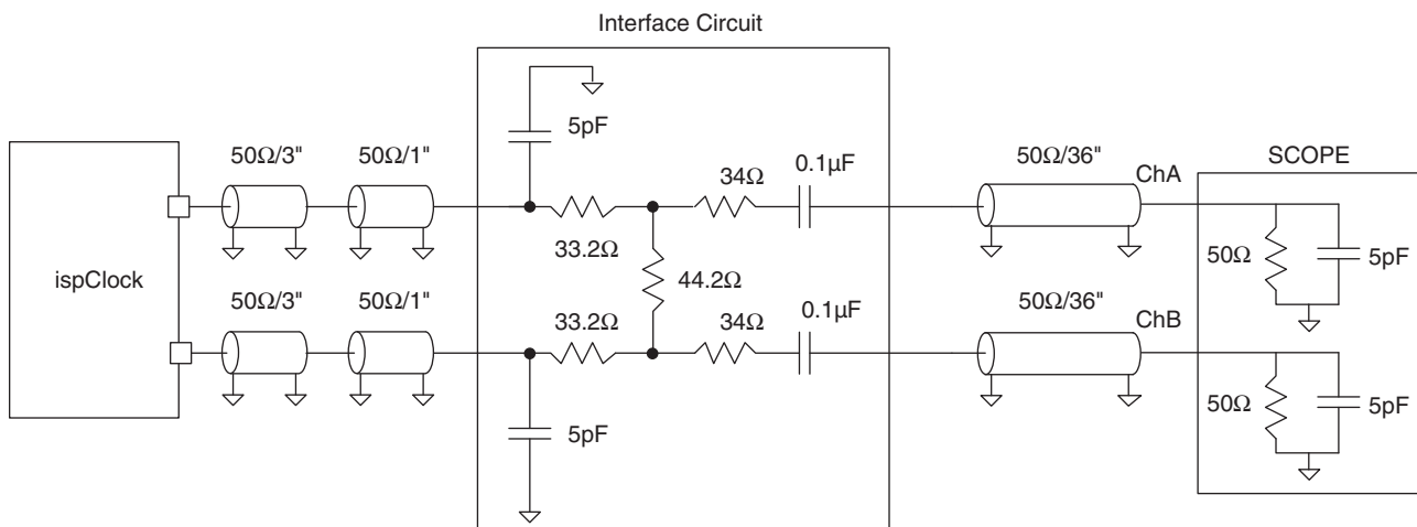
Figure 2-4. MLVDS Termination Load
