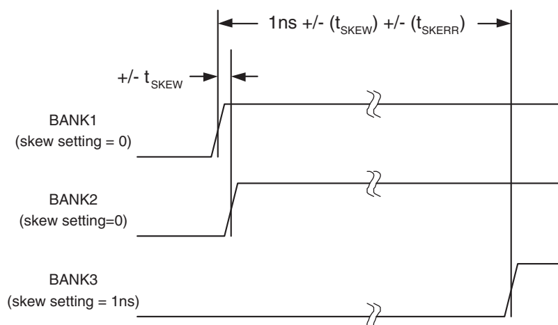
Figure 2-23. Skew Matching Error Sources
