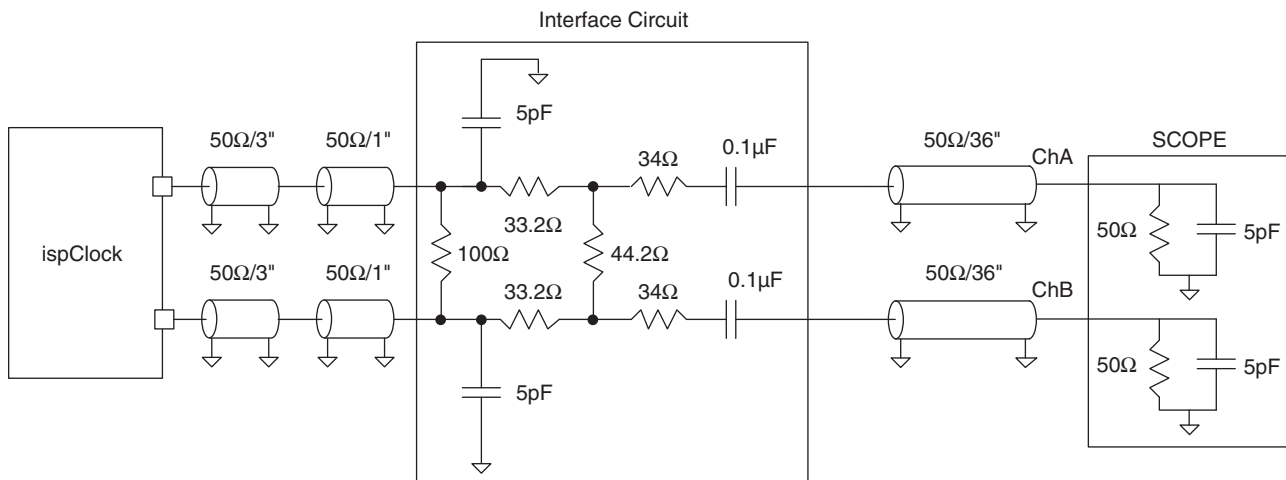
Figure 2-5. Differential HSTL Termination Load
