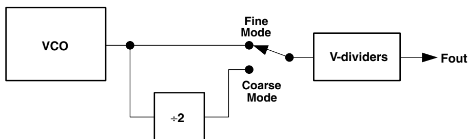
Figure 3-26. Additional Factor-of-2 Division in Coarse Mode
