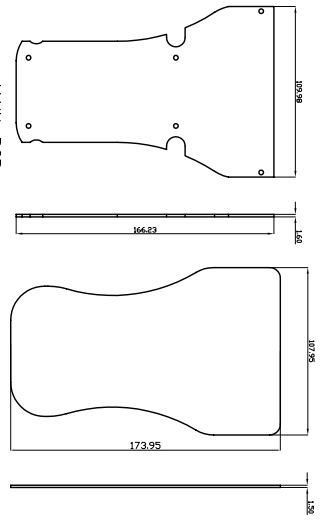
MAIN-PCB
