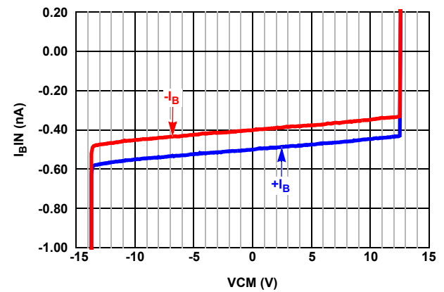
FIGURE 21. I_{BIN} vs INPUT COMMON-MODE VOLTAGE ( \pm 15V )
