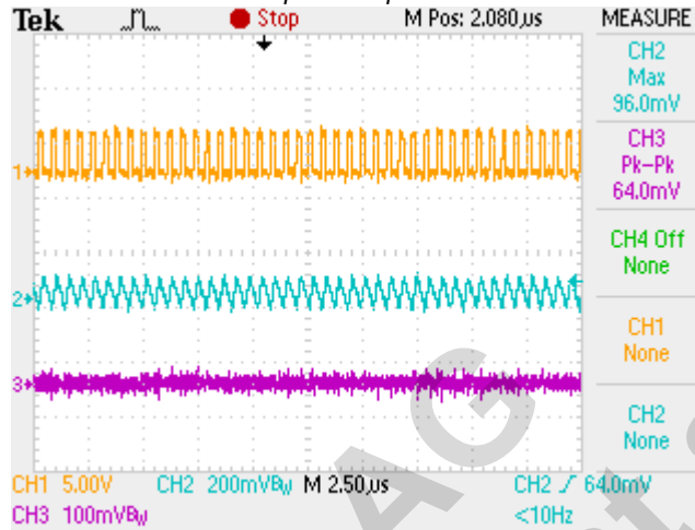
Figure 22. DCDC buck with disabled current force / pulse skip mode
