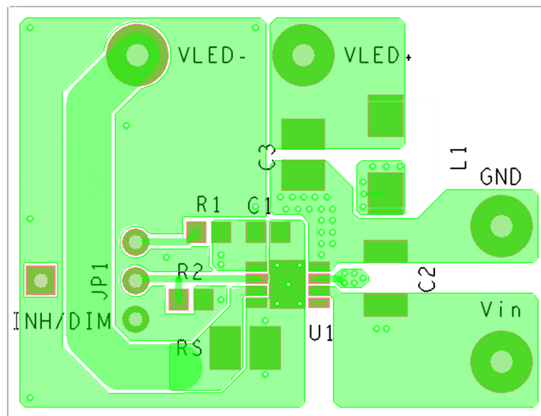
Figure 16. Layout example
