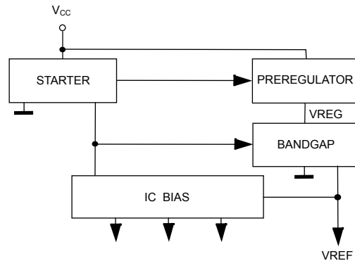
Figure 4. Internal circuit
