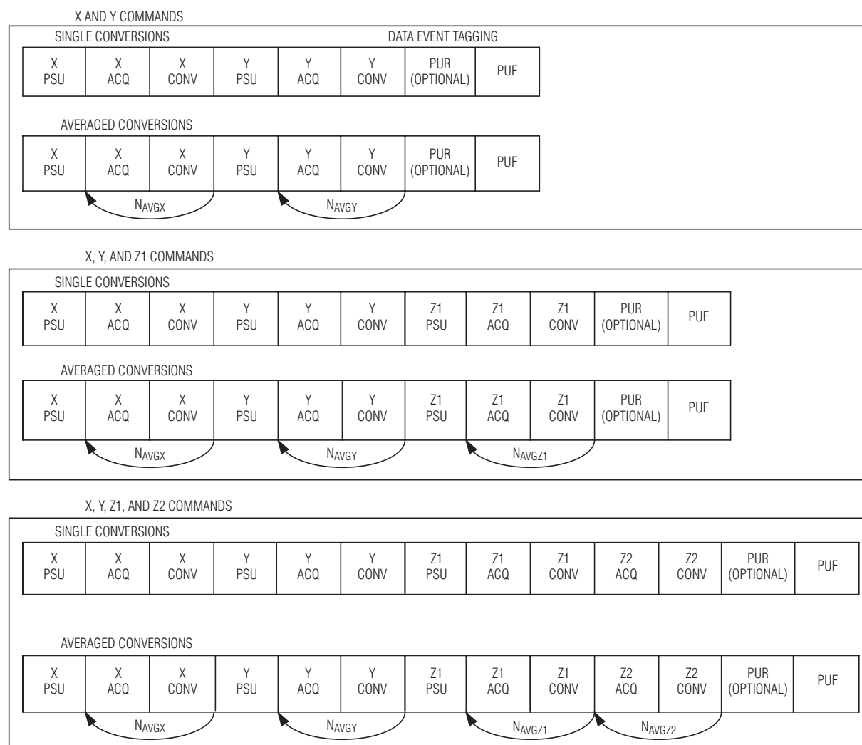
Figure 13. Combined Commands—MAX11800–MAX11803
