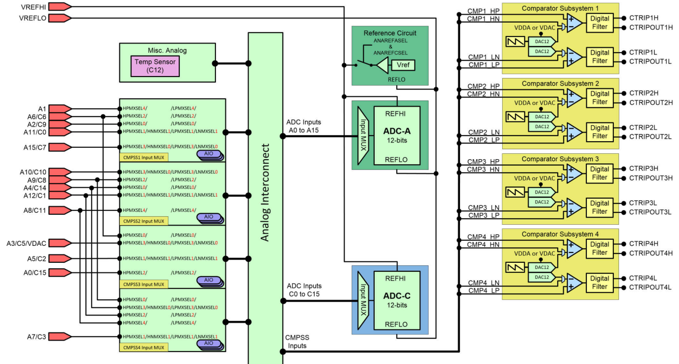
Figure 6-37. Analog Subsystem Block Diagram (48-Pin PT LQFP)
