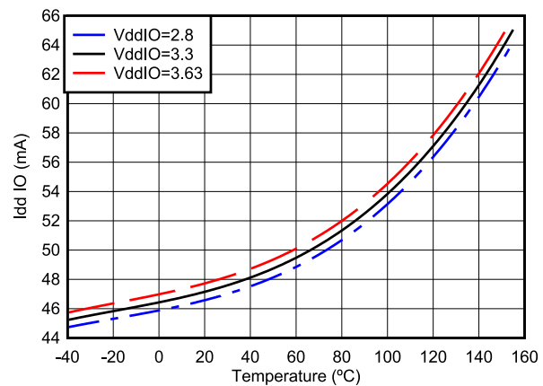
Figure 6-3. Operating Current Versus Temperature
