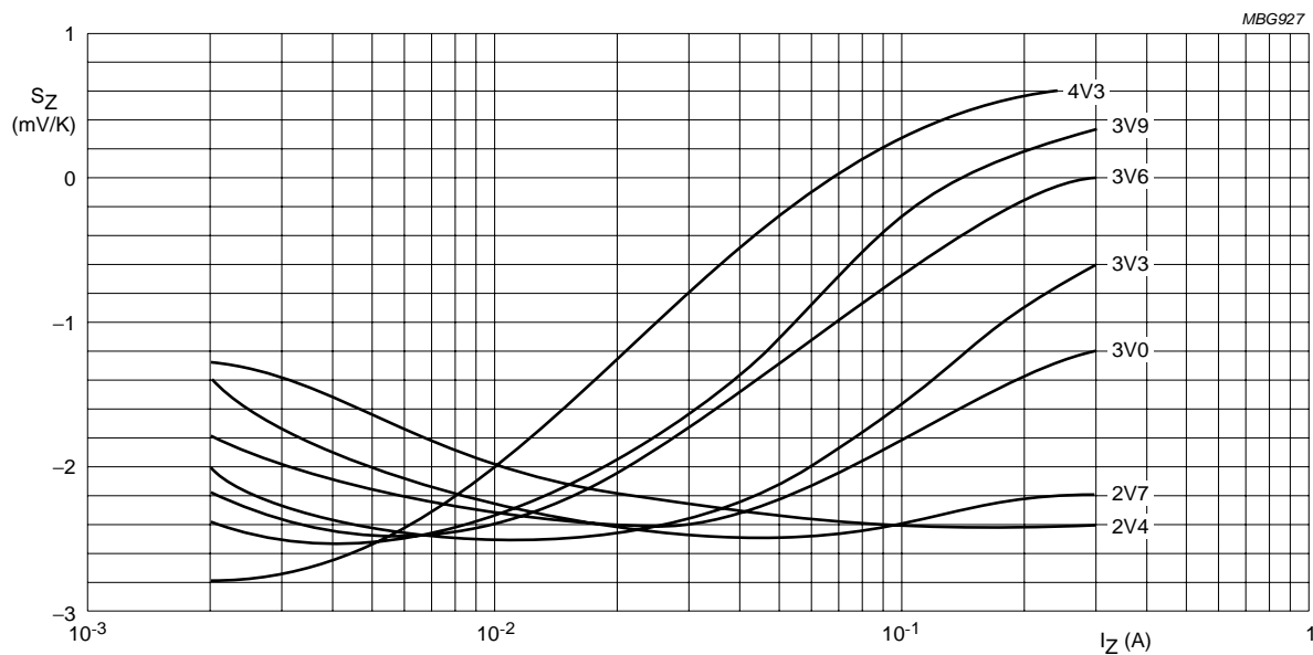
BZV90-C2V4 to C4V3. T_j = 25 to 150 °C.
