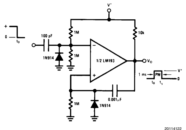
One-Shot Multivibrator
