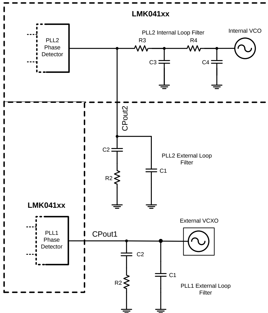
Figure 13. Loop Filter
