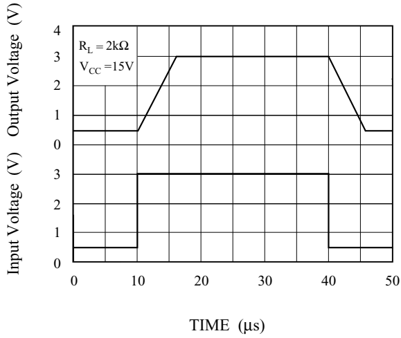
Fig. 7 Voltage Follower Pulse Response
