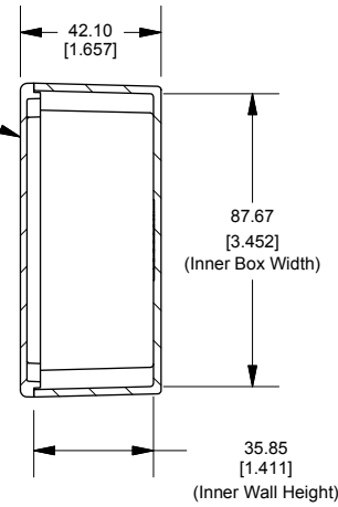
SECTION A-A End View of Assembly
