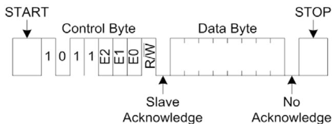
Figure 12-1. OTP Security Register Current Address Read
