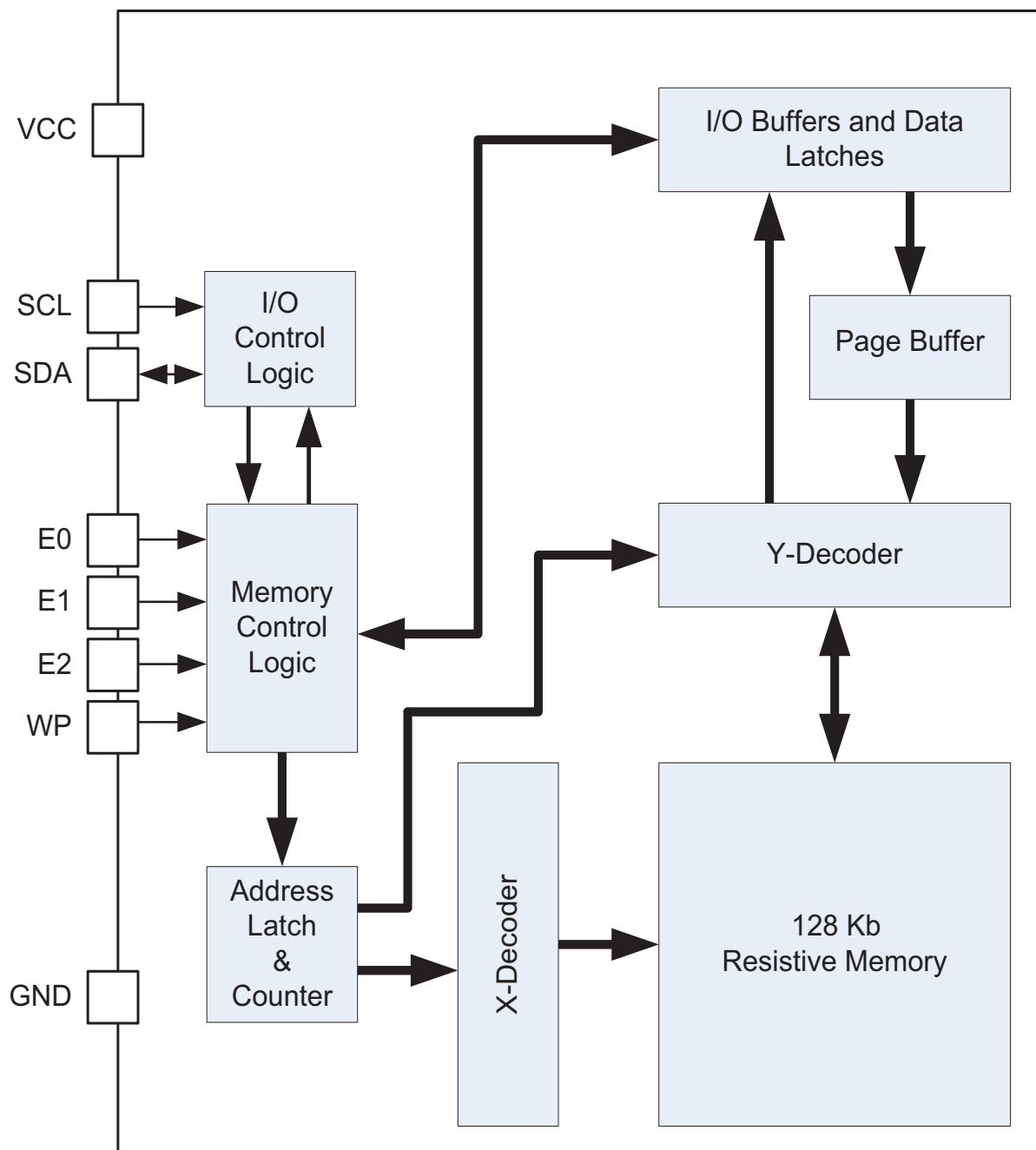
Figure 1-1. Block Diagram
