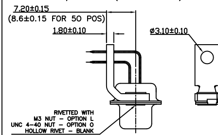
VIEW WITH RIVET &amp; METAL BRACKET
