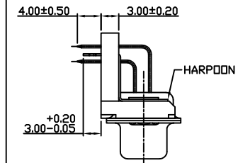
VIEW WITH RIVETED FEMALE SCREW &amp; METAL BRACKET
