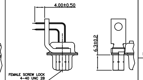
VIEW WITH RIVETED FEMALE SCREW &amp; METAL BRACKET
