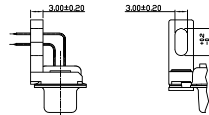
BRACKET DETAILS
