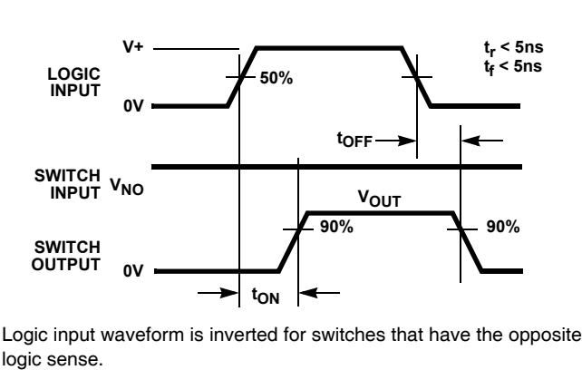
FIGURE 1A. MEASUREMENT POINTS
