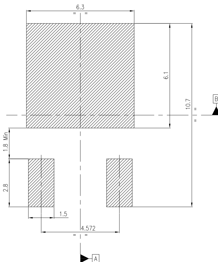
Figure 13. DPAK recommended footprint (dimensions are in mm)
