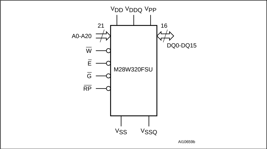
Figure 3. M28W320FSU logic diagram
