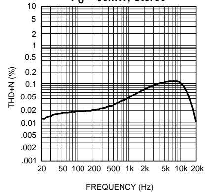
THD+N vs Frequency V_{DD} = 3.6V , R_L = 32\Omega , P_O = 60mW , Stereo
