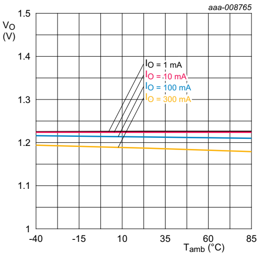
Fig 6. Temperature dependency of LD6835K/12x
