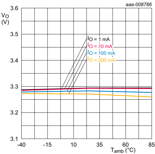
Fig 7. Temperature dependency of LD6835K/33x
