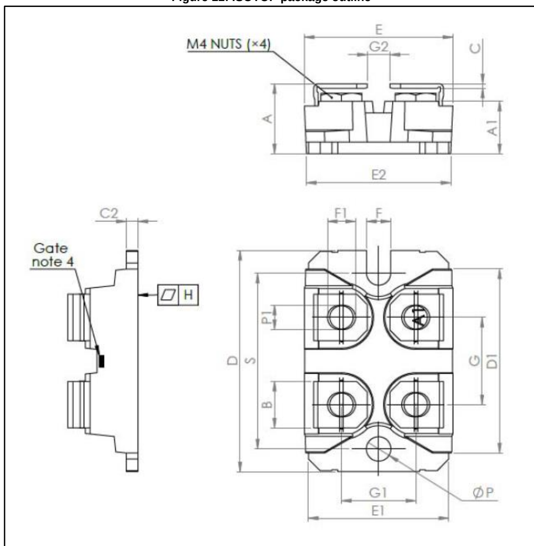
Figure 11: ISOTOP package outline
