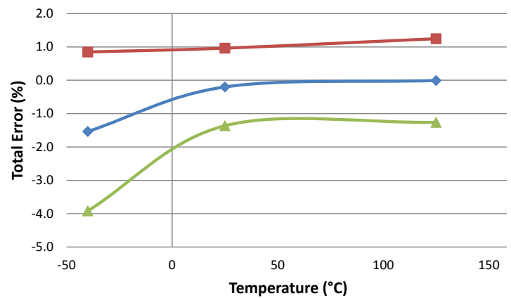
Total Error at I_{PR}(\text{max}) vs. Temperature
