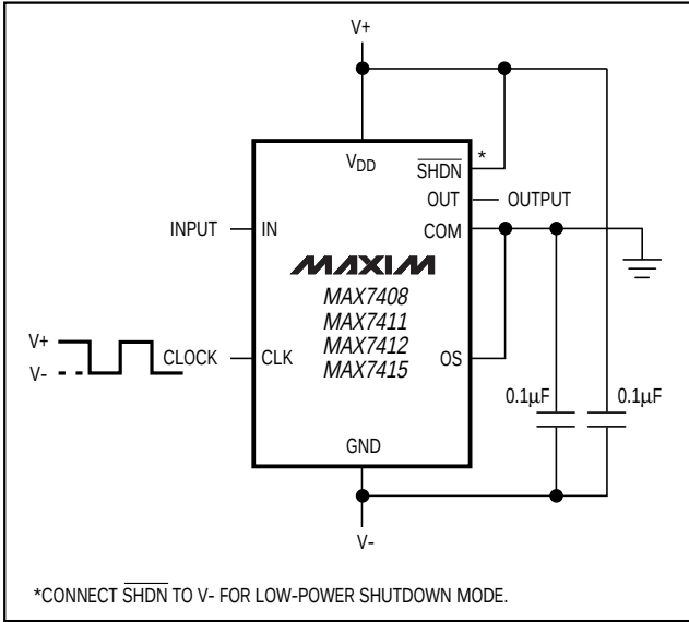
Figure 4. Dual-Supply Operation
