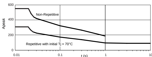
Figure 5c — SD48 50A output current
