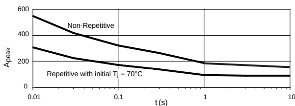
Figure 5a — SD24 50A output current
