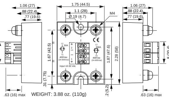
Figure 2e — SD48D50A2; dimensions in inches (mm)
