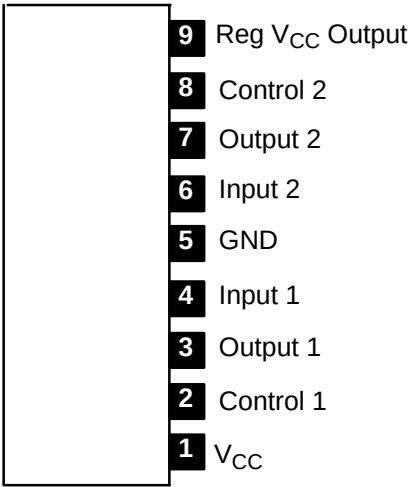
Pin Connection Diagram
