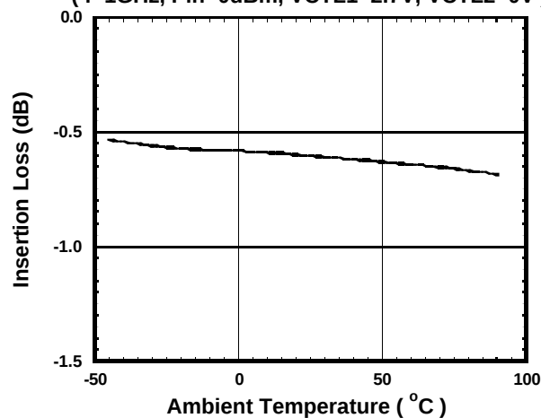
PC-P2 Loss vs. Ambient Temperature
