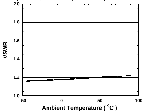
P1 VSWR vs. Ambient Temperature
