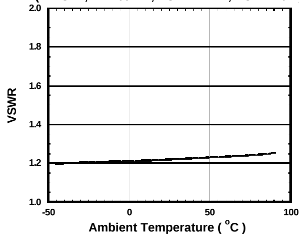
P2 VSWR vs. Ambient Temperature
