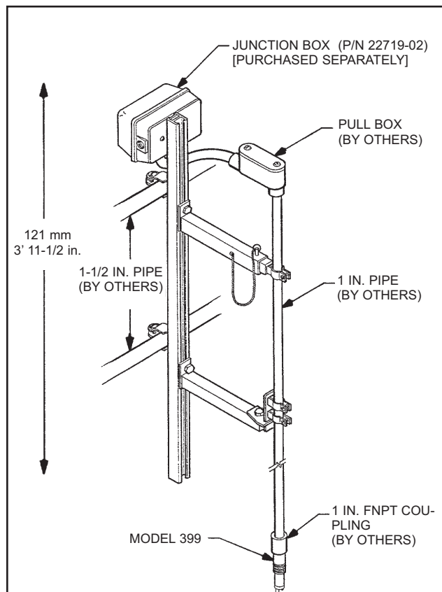
HANDRAIL MOUNTING ACCESSORY (P/N 1000857)
