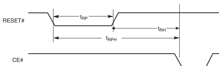
Figure 13.1 Reset Timings
