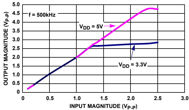
FIGURE 9. MAXIMUM OUTPUT MAGNITUDE vs INPUT MAGNITUDE
