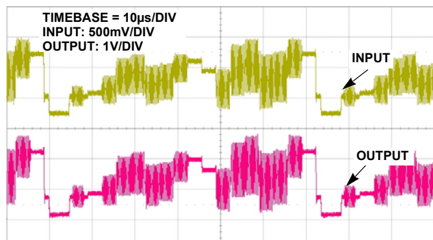
FIGURE 15. NTSC COLOR BAR
