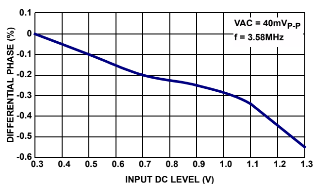
FIGURE 18. DIFFERENTIAL PHASE
