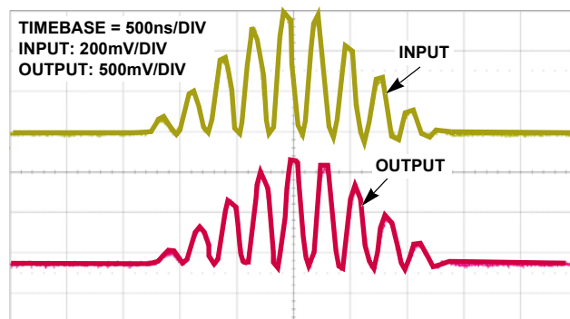
FIGURE 14. 12.5T RESPONSE
