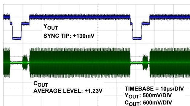
FIGURE 16. S-VIDEO OUTPUT
