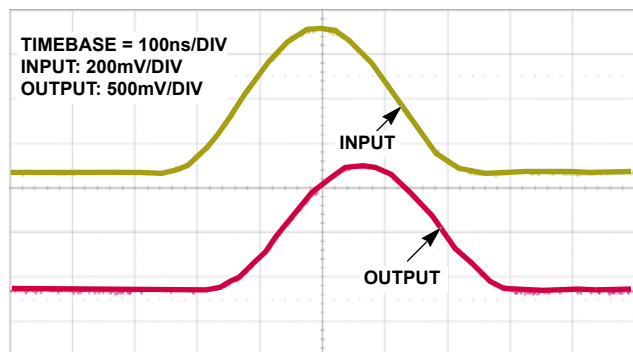
FIGURE 13. 2T RESPONSE
