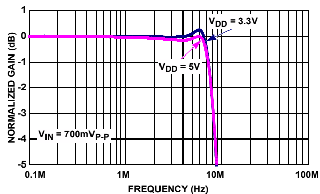
FIGURE 2. LARGE SIGNAL GAIN vs FREQUENCY -0.1dB
