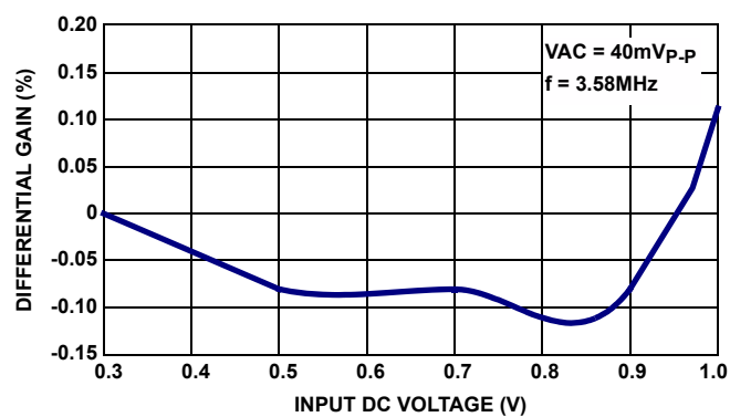
FIGURE 17. DIFFERENTIAL GAIN
