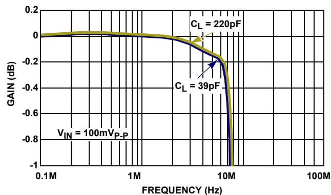
FIGURE 4. GAIN vs FREQUENCY FOR VARIOUS C_{LOAD}
