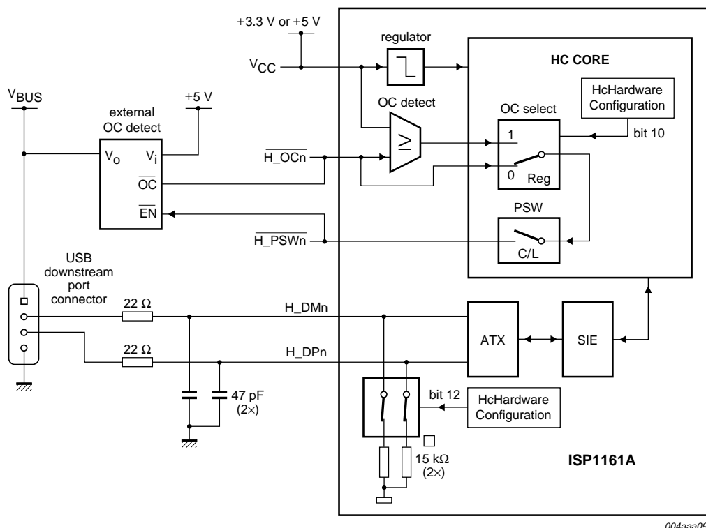
Fig 35. Using an external OC detection circuit.
