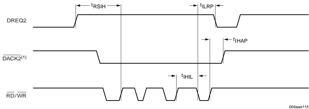
Fig 60. DC burst mode DMA timing.
