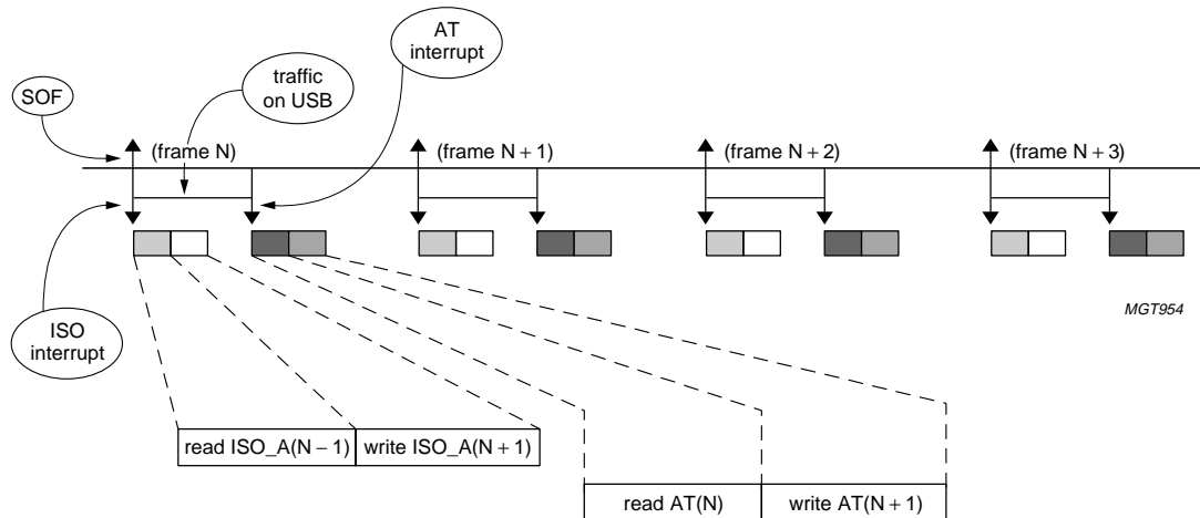
Fig 29. HC time domain behavior: example 1.
