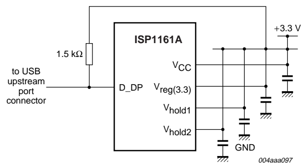
Fig 44. Using a +3.3 V supply.
