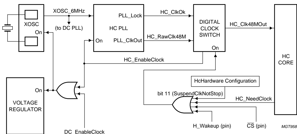
Fig 36. ISP1161A suspend and resume clock scheme.
