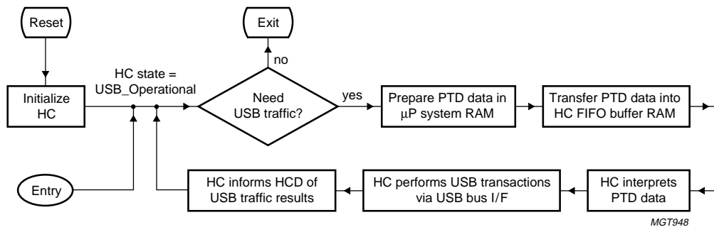
Fig 23. ISP1161A HC USB transaction loop
