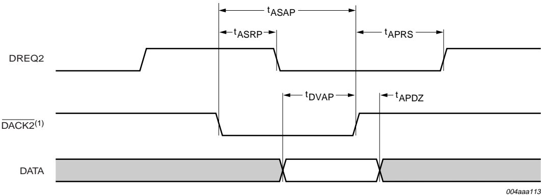
Fig 58. DC single-cycle DMA write timing in DACK-only mode.
