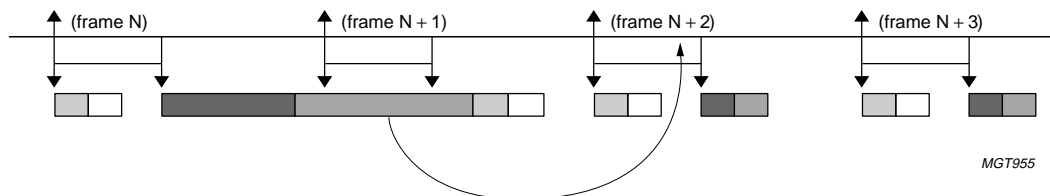
Fig 30. HC time domain behavior: example 2.
