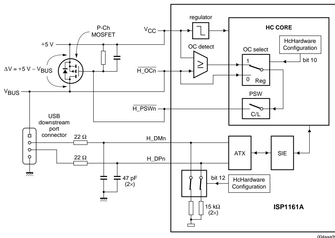
Fig 34. Using internal OC detection circuit.
