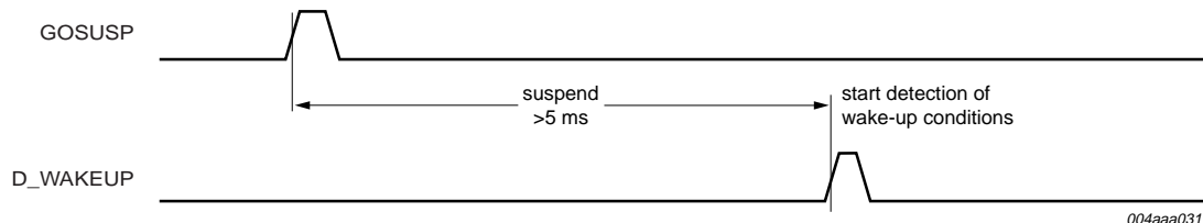
Fig 37. DC typical suspend timing.
