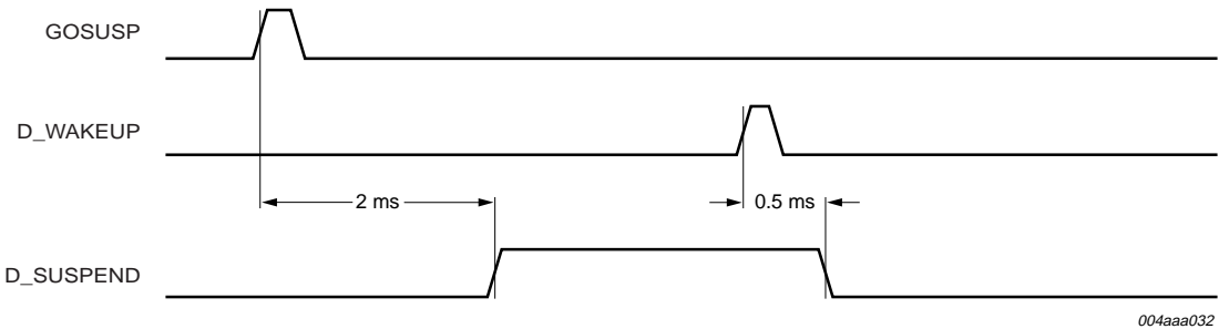
Fig 38. Suspend and resume timing for powered-off application (DC side).
