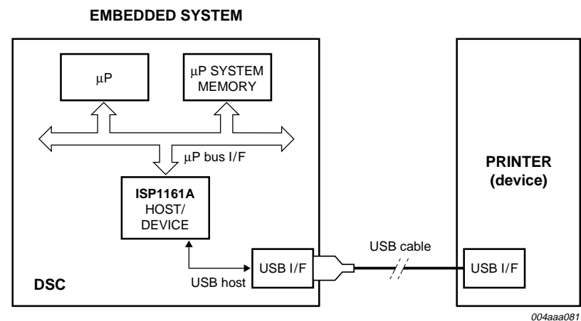
Fig 2. ISP1161A operating as a stand-alone USB host.
