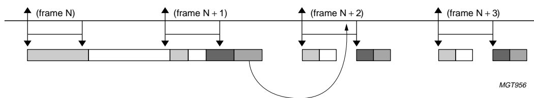
Fig 31. HC time domain behavior: example 3.
