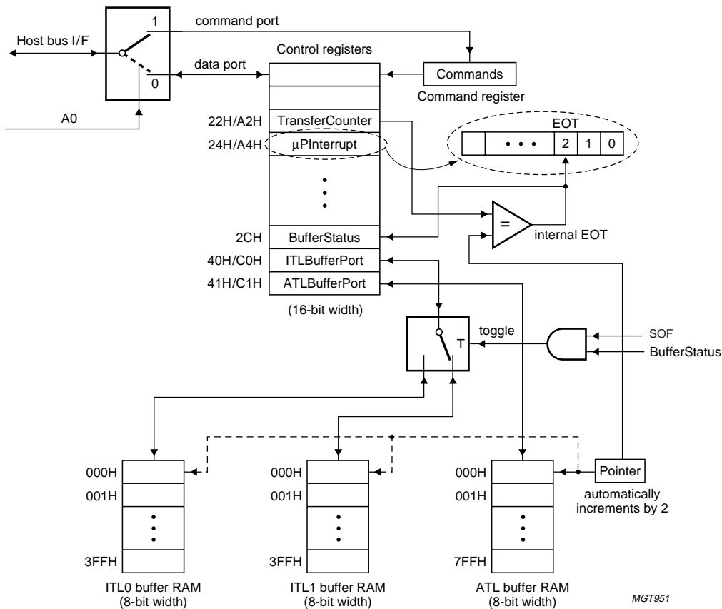
Fig 28. PIO access to internal FIFO buffer RAM.
