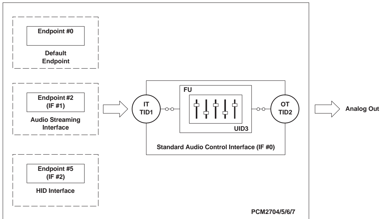
Figure 21. USB Audio Function Topology
