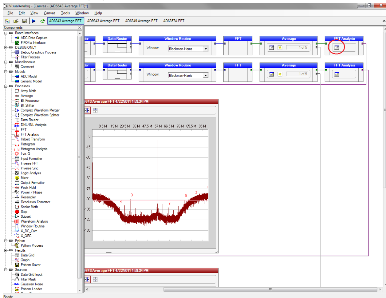
Figure 20. VisualAnalog, Main Window—Showing FFT Analysis for AD6643
