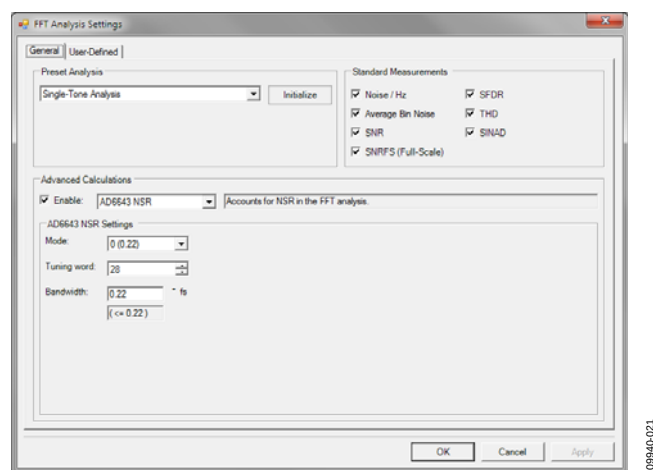
Figure 21. VisualAnalog, FFT Analysis Settings for AD6643
