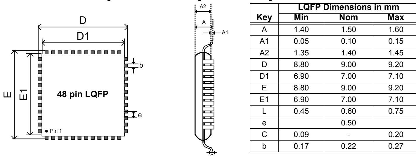
Figure 4. 48-Pin LQFP Package Outline and Package Dimensions
