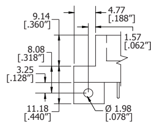
STRADDLE MOUNT (Q)
