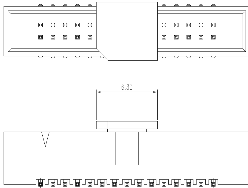
CONFIG 1: 20021521-001XXXXLF WITH EDGE CUT CAP, OTHER DIMENSIONS SEE SHEET 1
